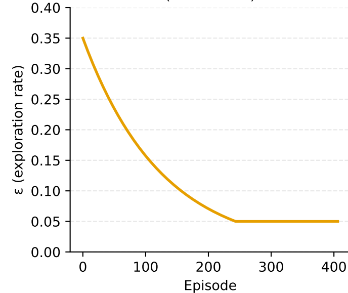
\epsilon Decay Schedule (0.35 \rightarrow 0.05)
