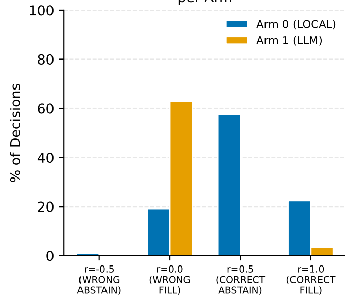
Reward Distribution per Arm
