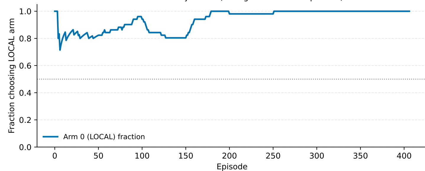
Arm Selection Dynamics (sliding window = 50 episodes)
