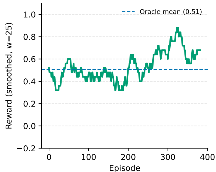
Bandit Reward over Episodes
